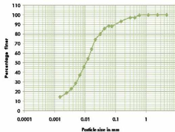
Fig 5: Grain size Distribution for Granite fines
